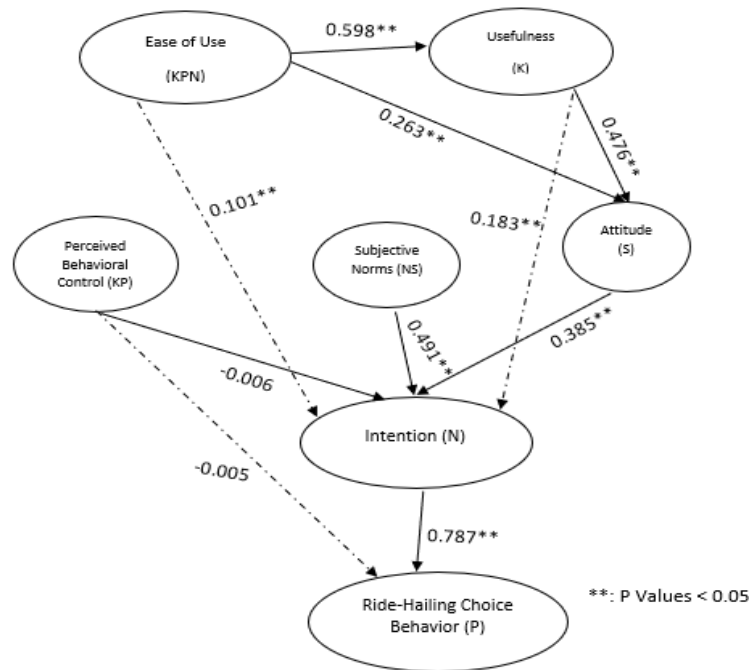
Figure 4. Hypothesis testing
