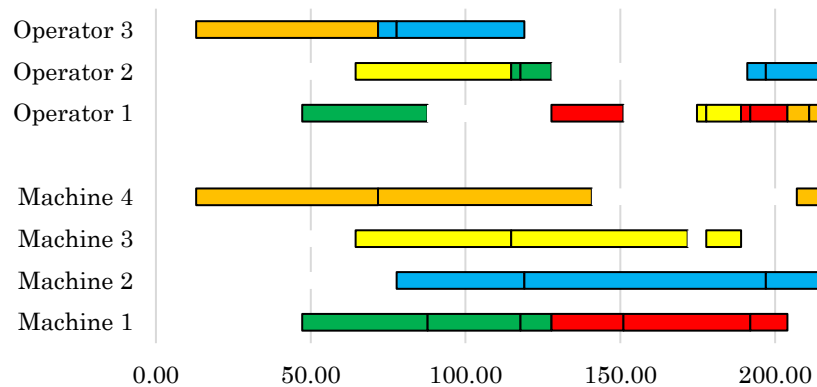
Figure 3. Gantt chart of MIQCP model
