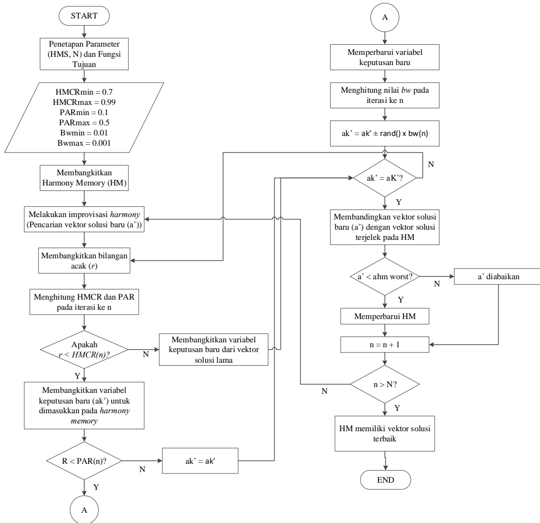
Gambar 4. Flowchart algoritma harmony search
